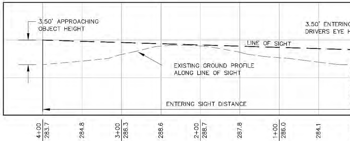
PROFILE EXAMPLE
