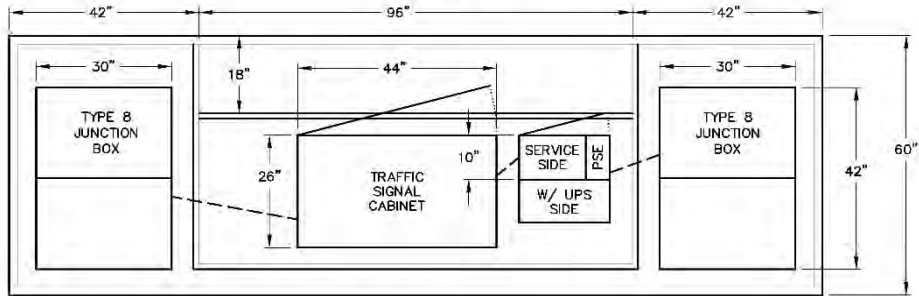
PLAN VIEW
