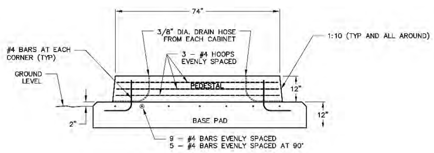
PROFILE VIEW
