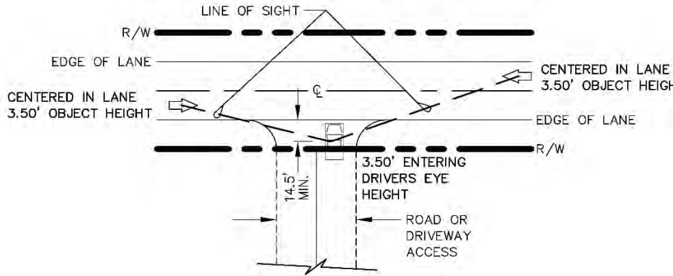
SIGHT DISTANCE DETAIL
