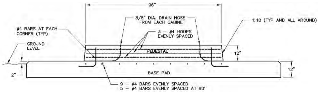
PROFILE VIEW
